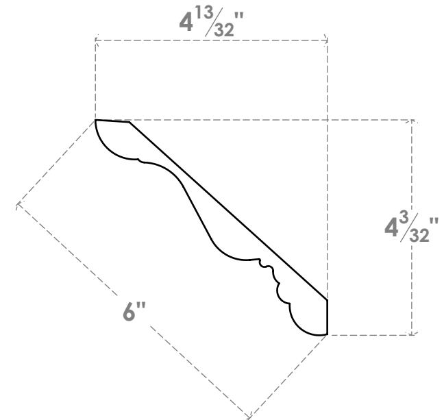
SIDE PROFILE
