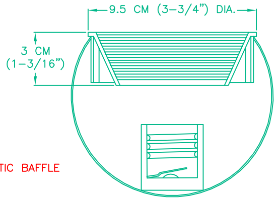
SECTIONED VIEW
