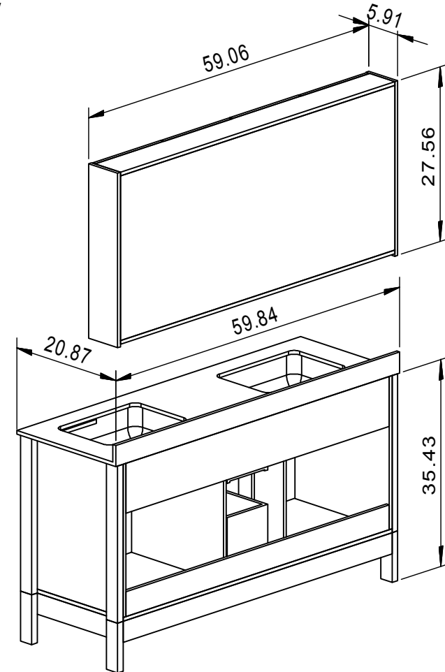
Back View
