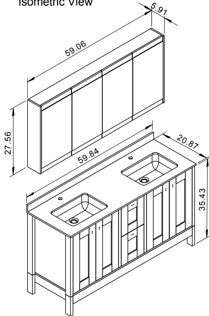
Isometric View
