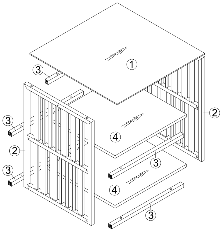
Exploded View
