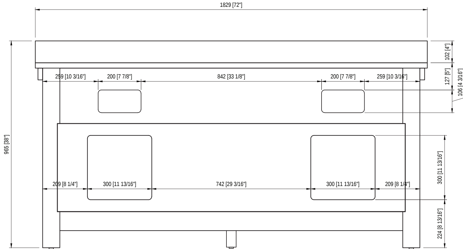
BACK VIEW
