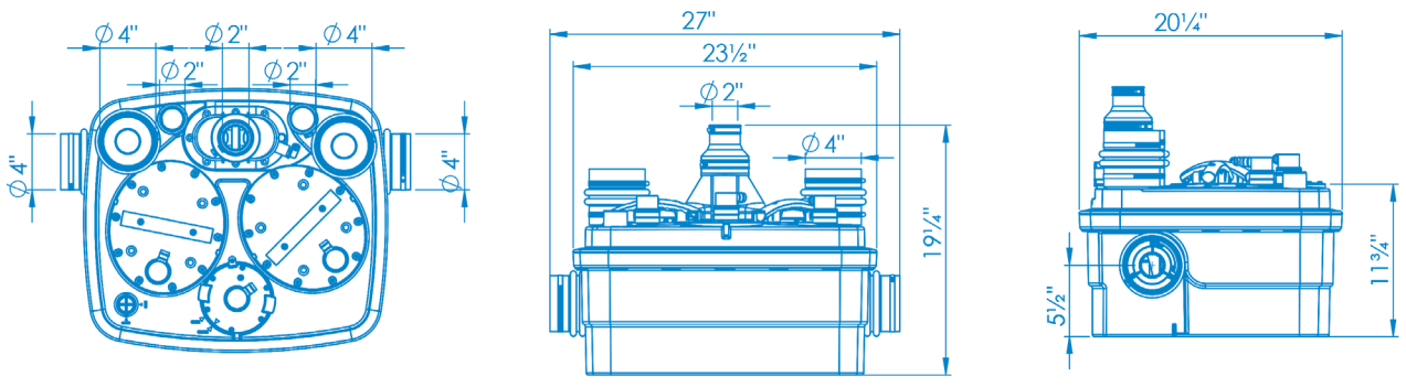
SANICUBIC® 2 - sizing diagram
