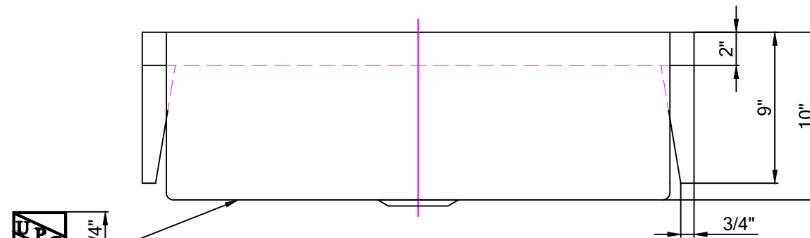
Side section view
