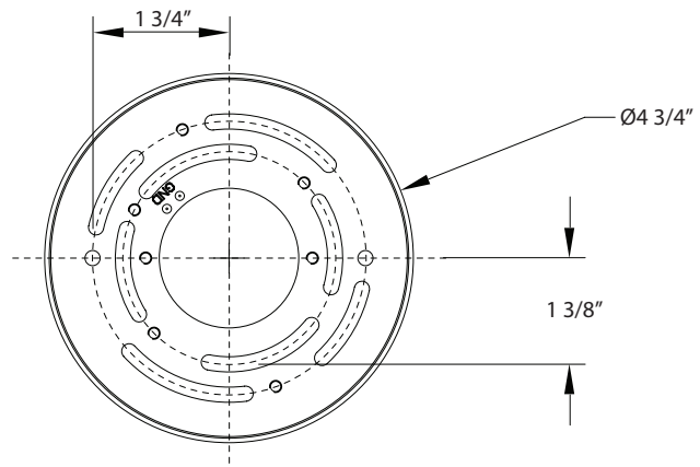
Back Plate Dimensions
