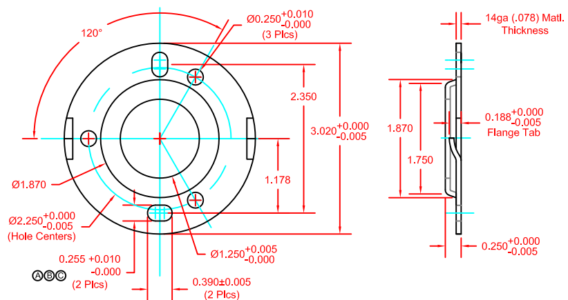
IQCR5-D-Flange_c Concealed Flange Detail
