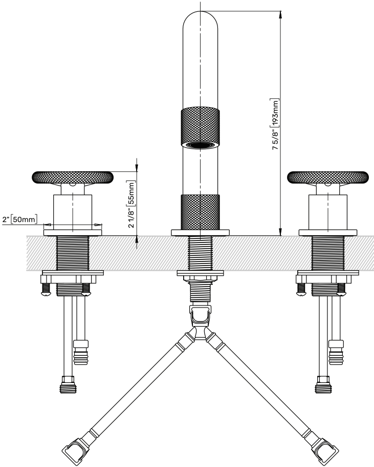
FRONT VIEW / VISTA FRONTAL / VUE DE FACE
