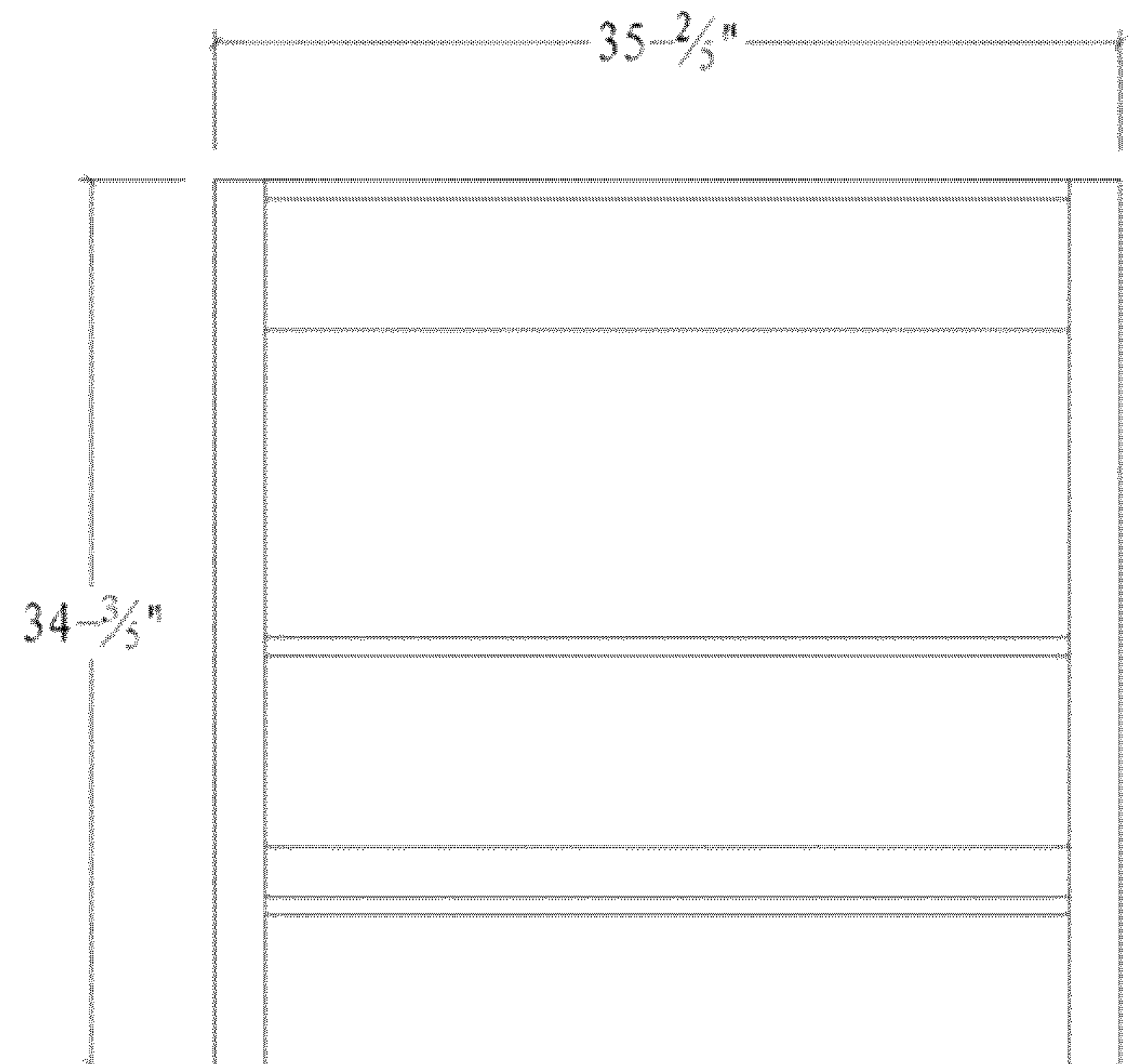
BACK VIEW
