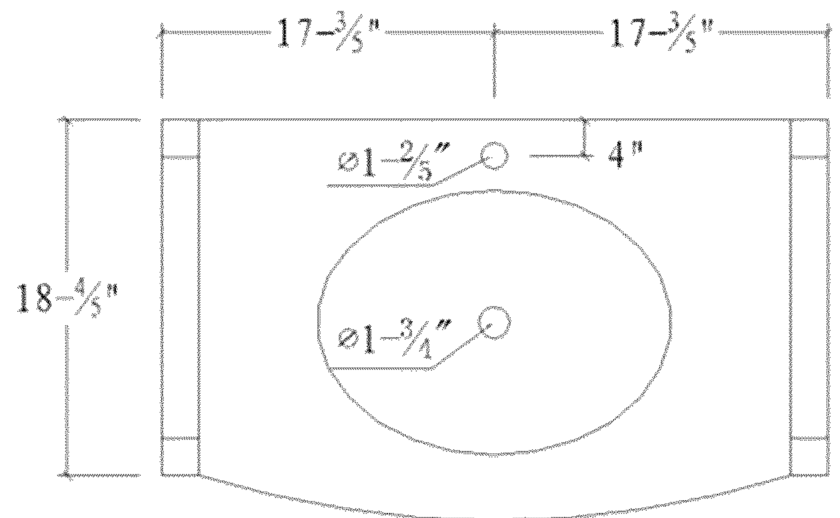
TOP VIEW
