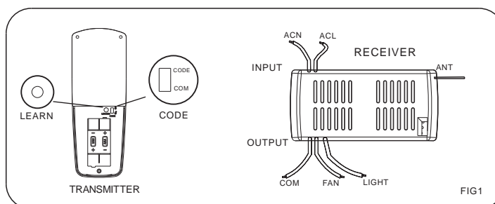
MODEL: GA012 OPERATION DISTANCE 20 FEET
