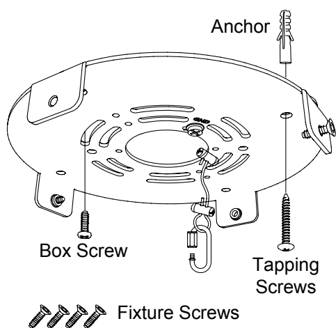
Mounting Plate
