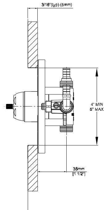
THIN WALL
