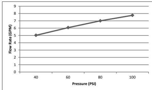
P-2301B Flow Rate (GPM) Vs Pressure (PSI) For Tub Port*
