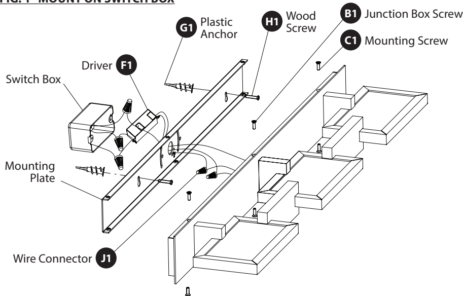
FIG. 1 MOUNT ON SWITCH BOX
