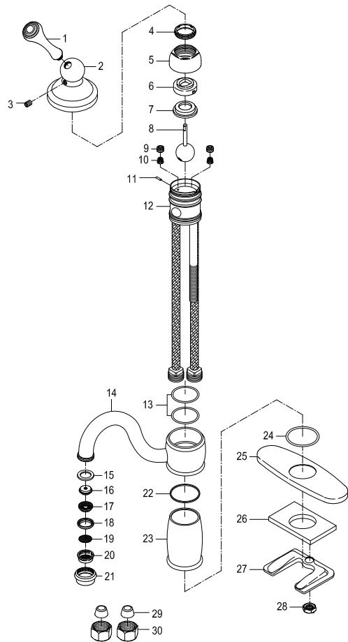
Cartridge: KBRP521C
