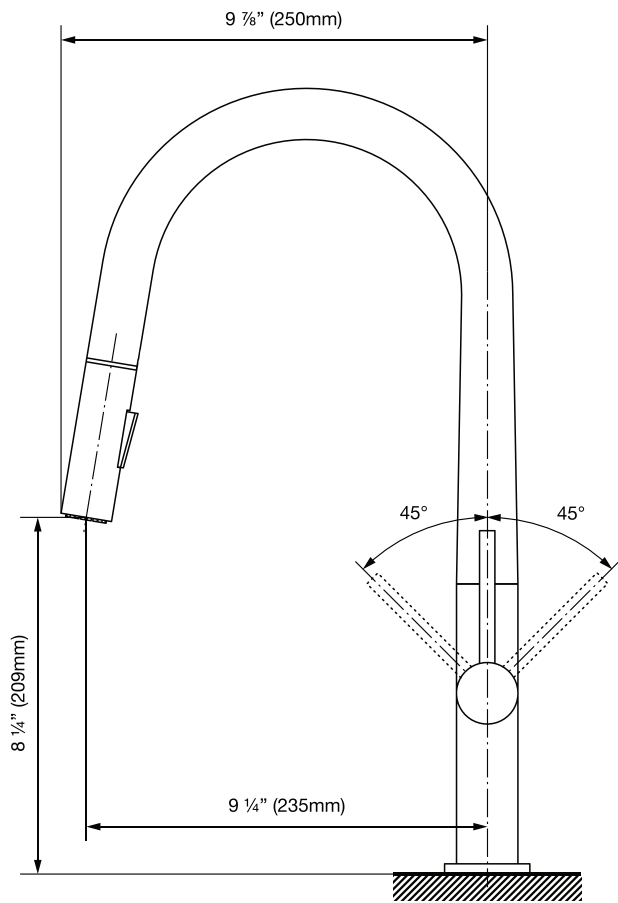
FRONT VIEW / VISTA FRONTAL / VUE DE FACE
