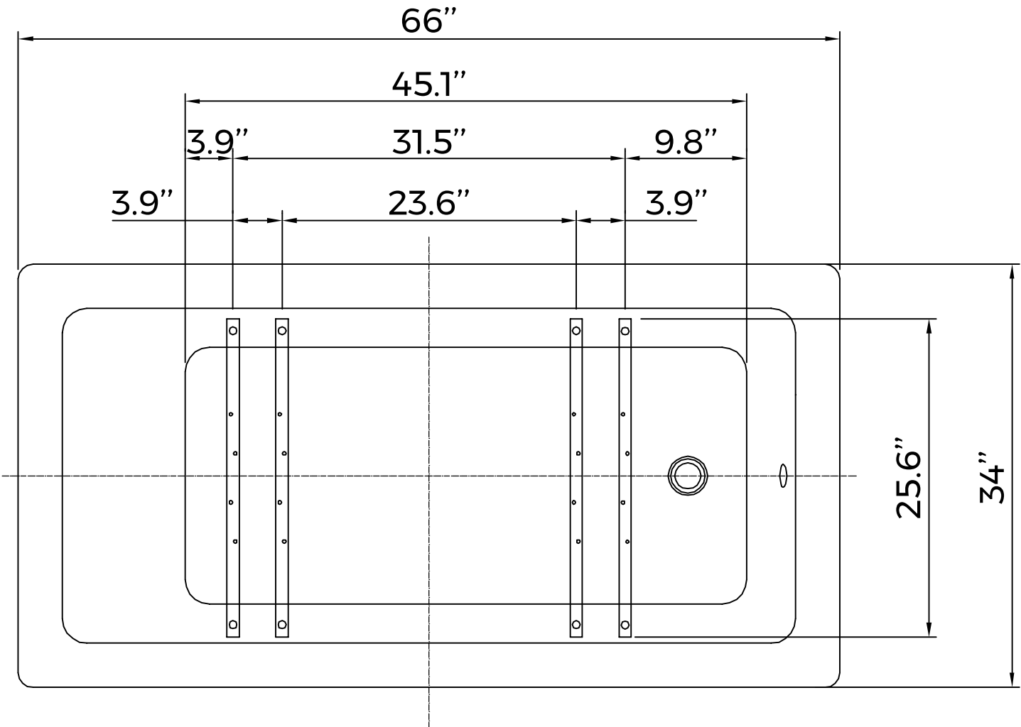
Leveling Foot Placement
