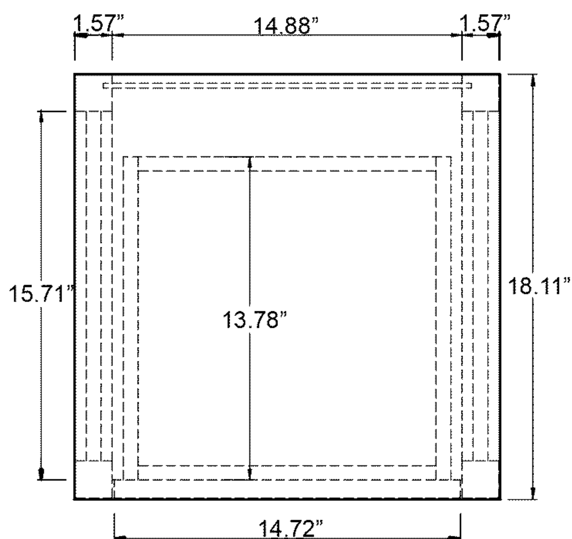
Top View
