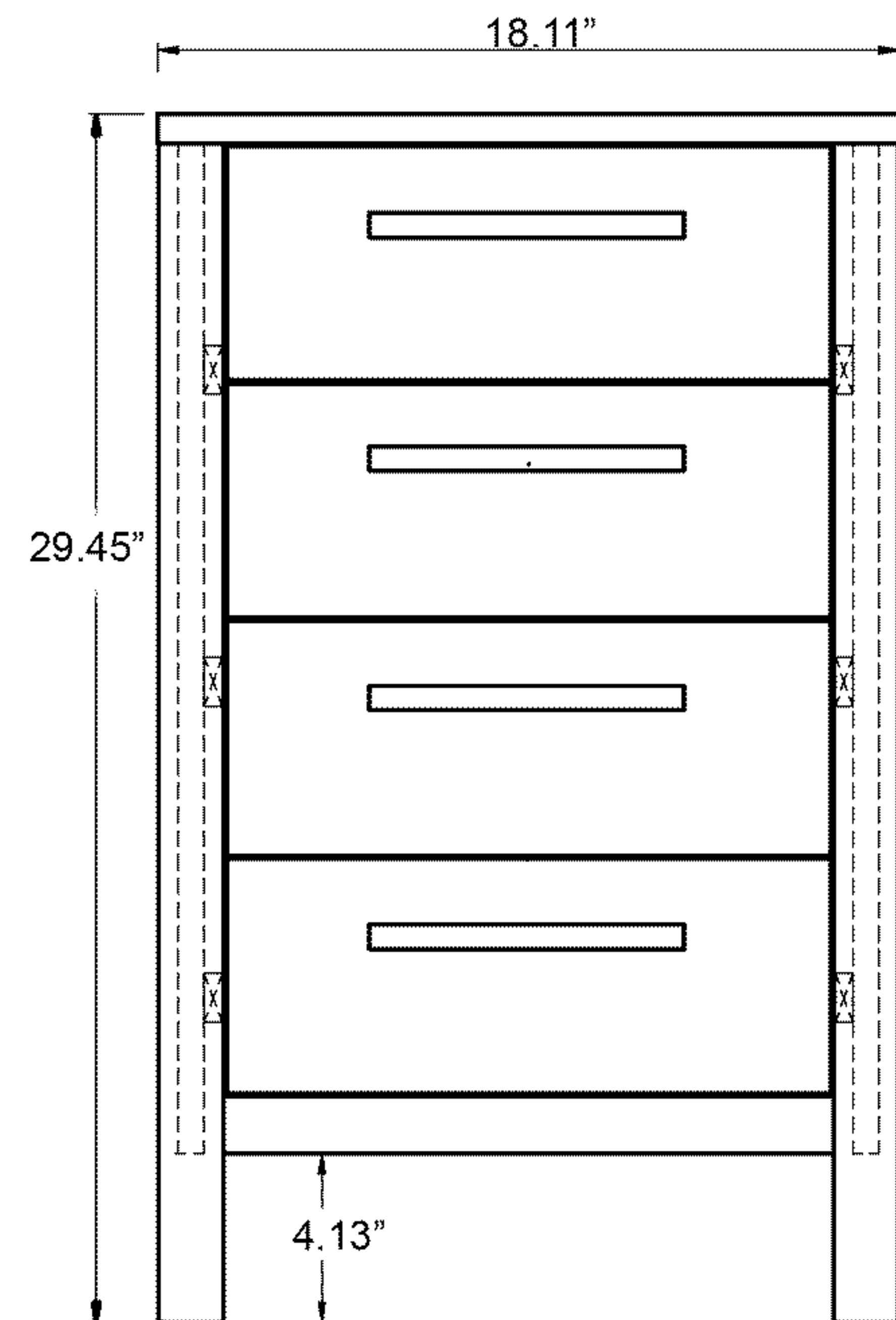
Front View
