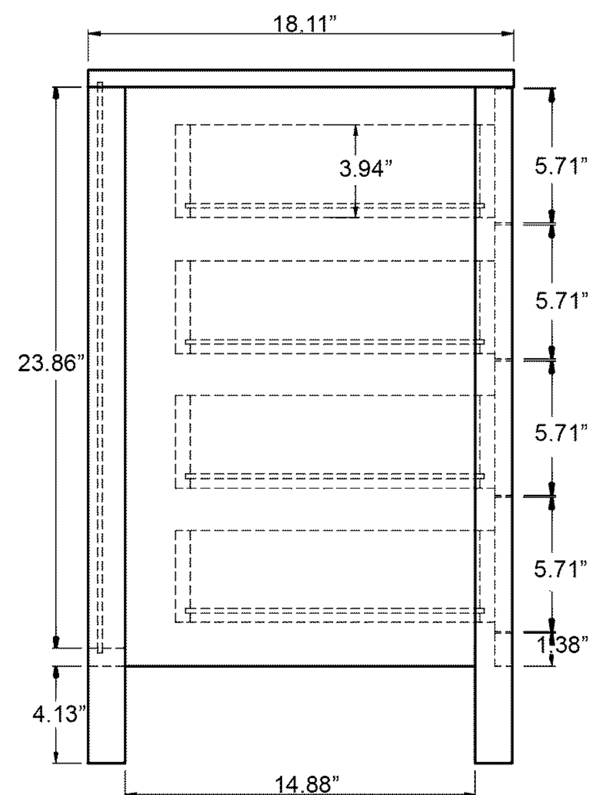
Side View
