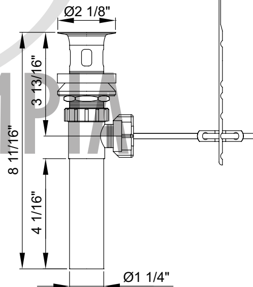
50/50 Pop-Up Drain
