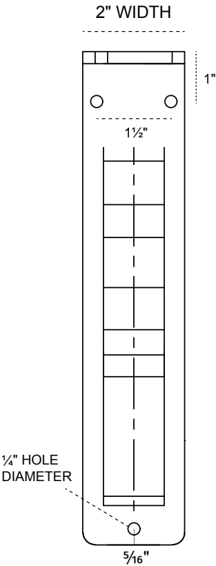
FRONT PROFILE
