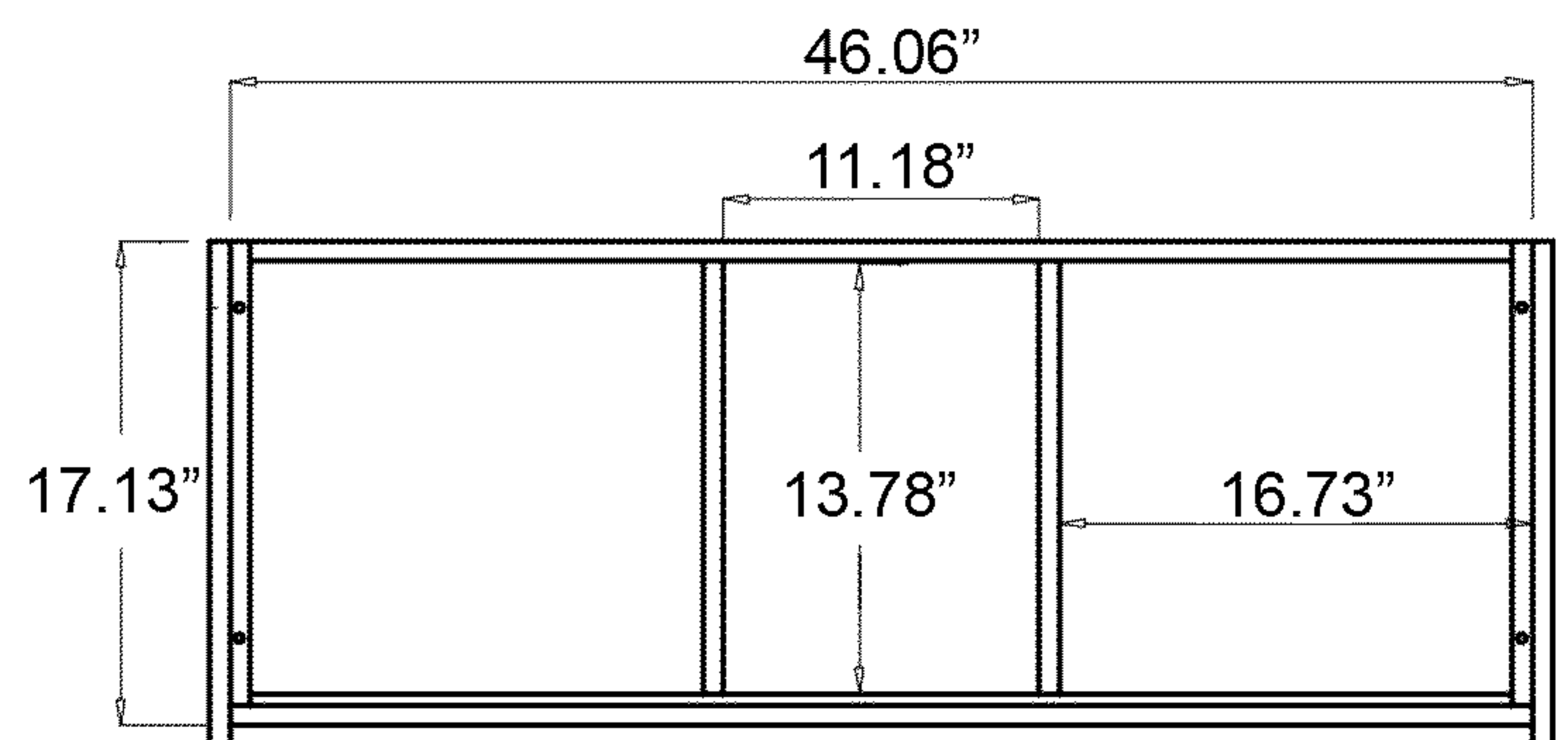
Top View
