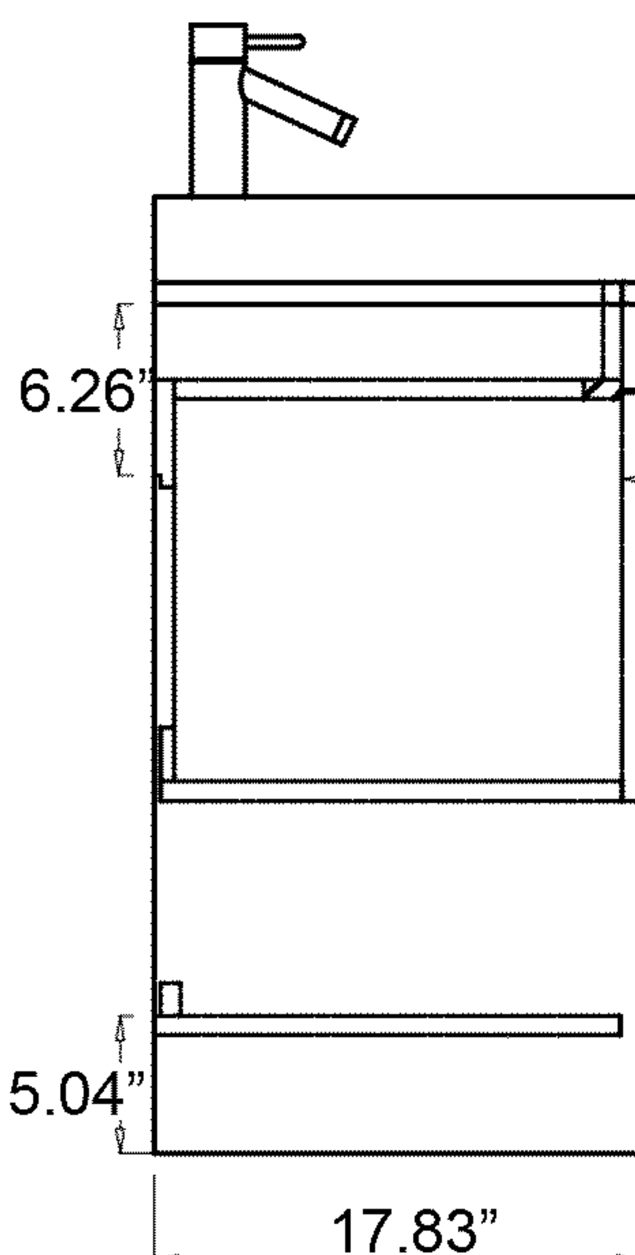
Side View
