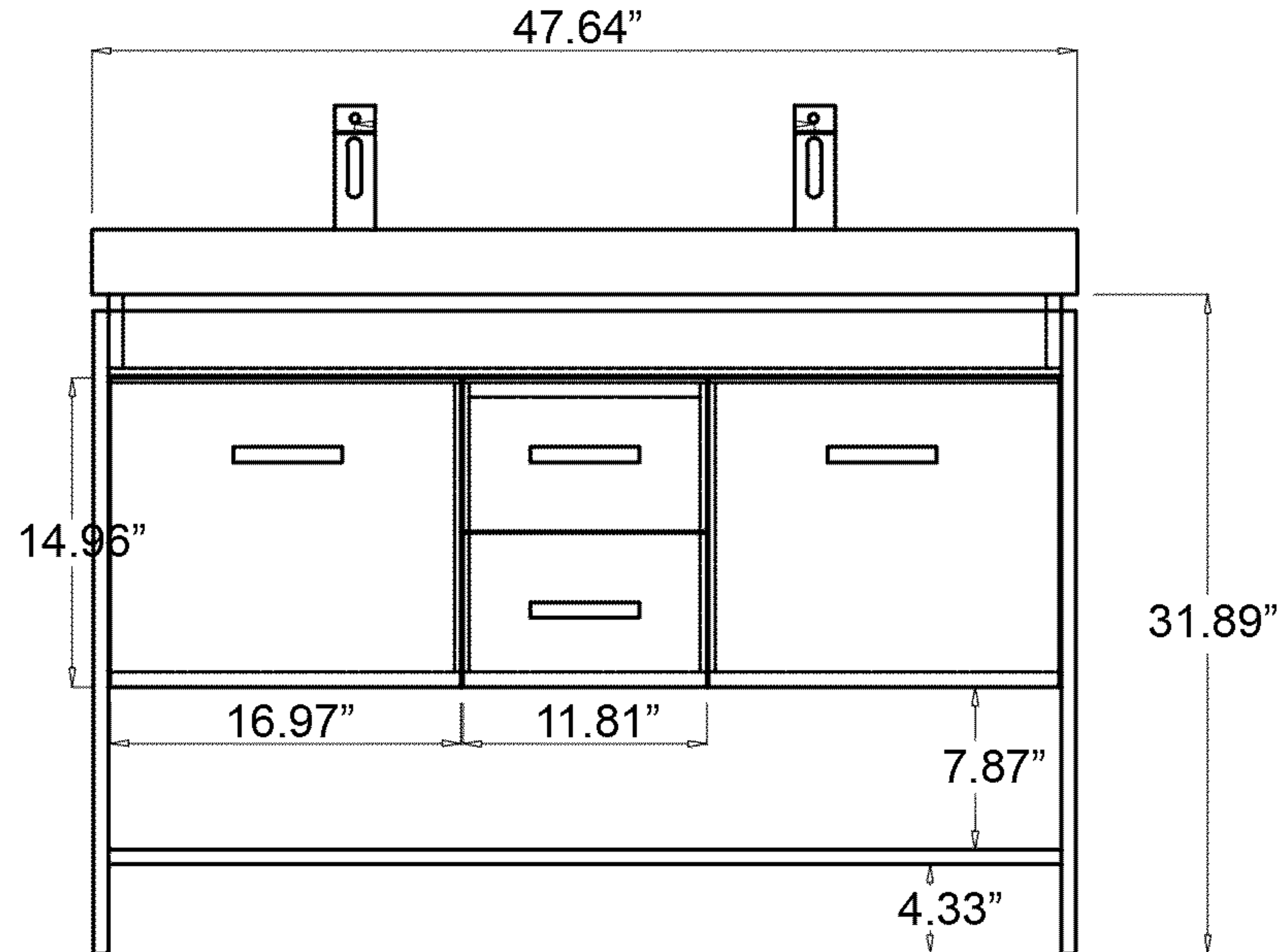
Front View
