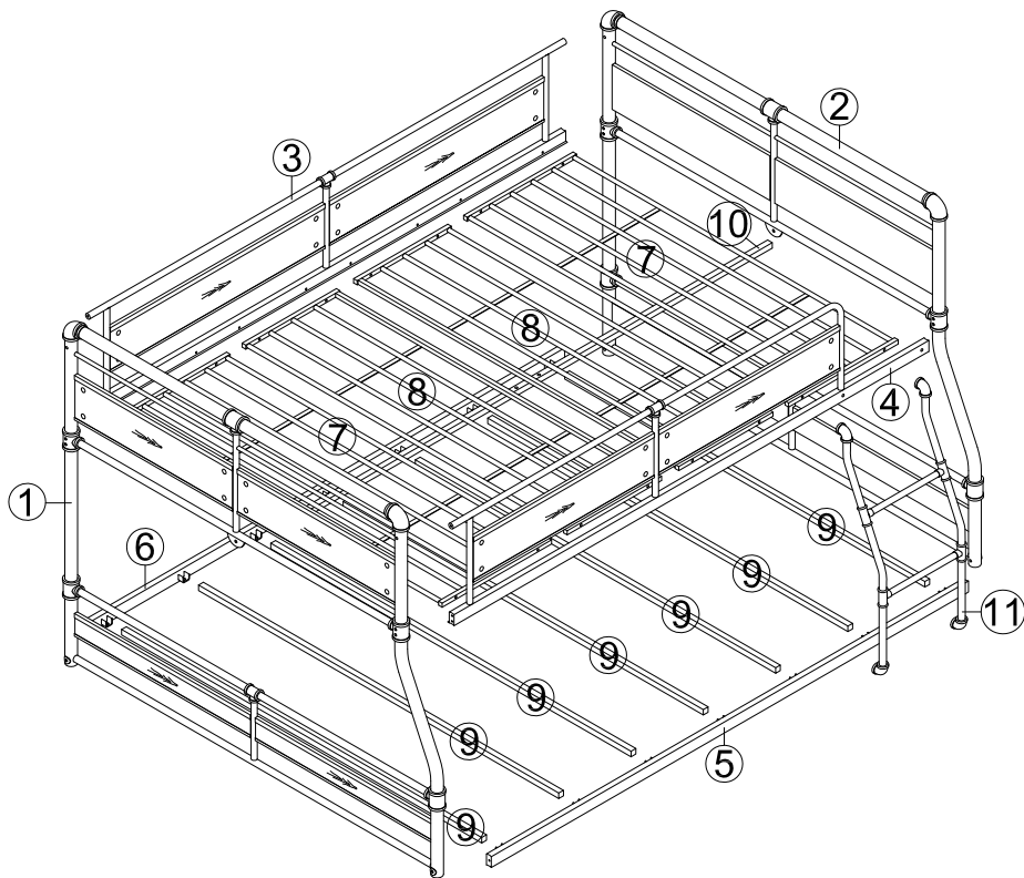
Exploded View
