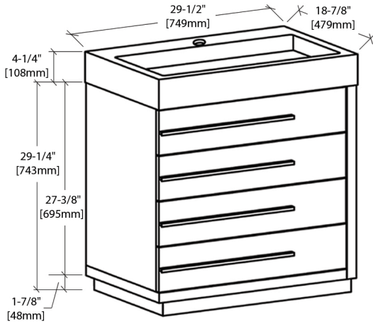
VANITY FRONT VIEW (V8005 30)
