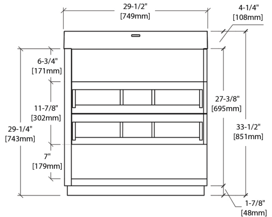
VANITY BACK VIEW (V8005 30)
