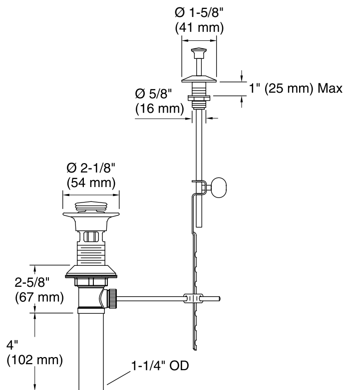
Pop-Up Drain
