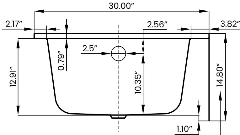
Height including Integral Flange
