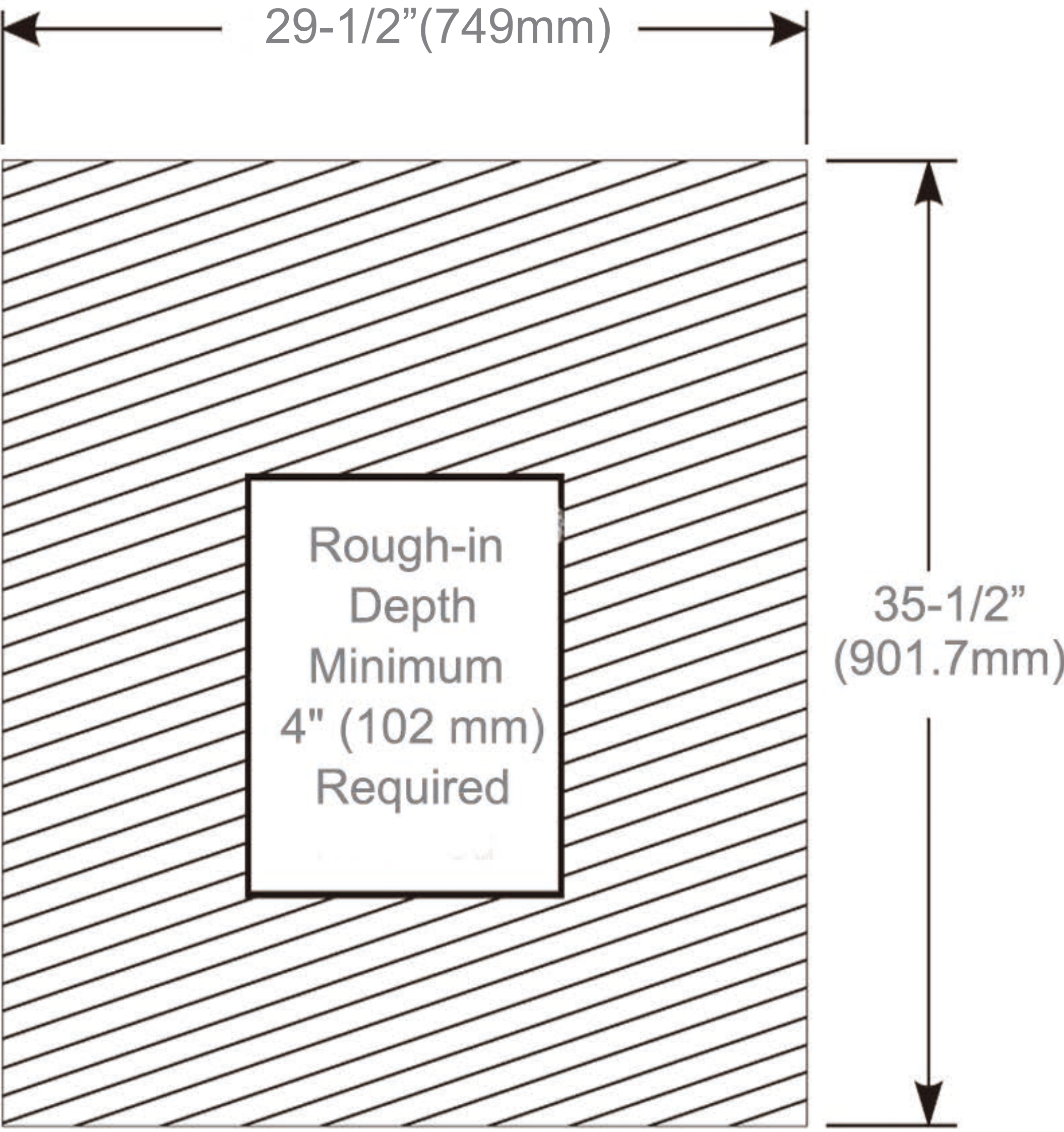
Rough-in Dimensions
