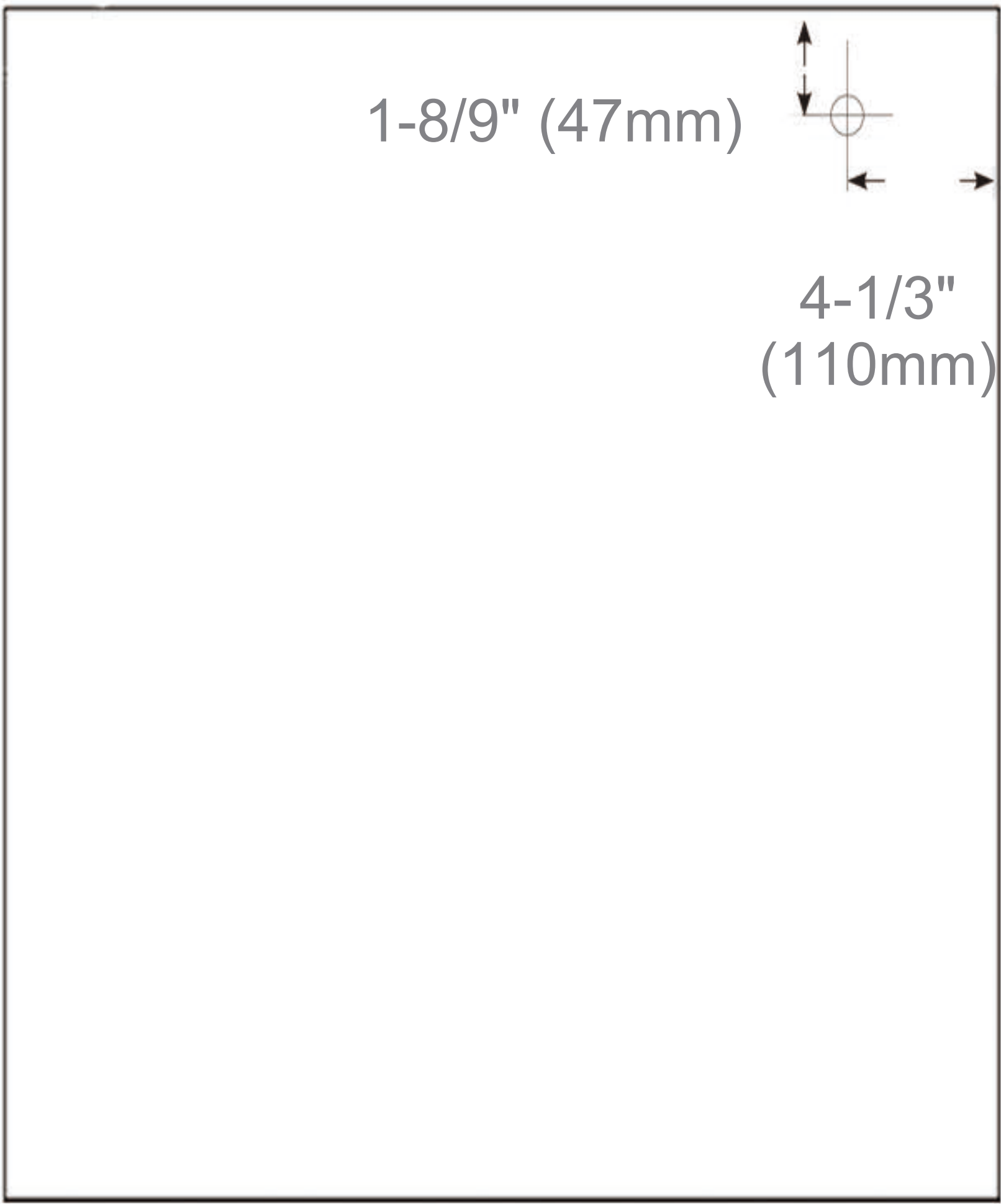
Back of Cabinet - Wire Access Location
