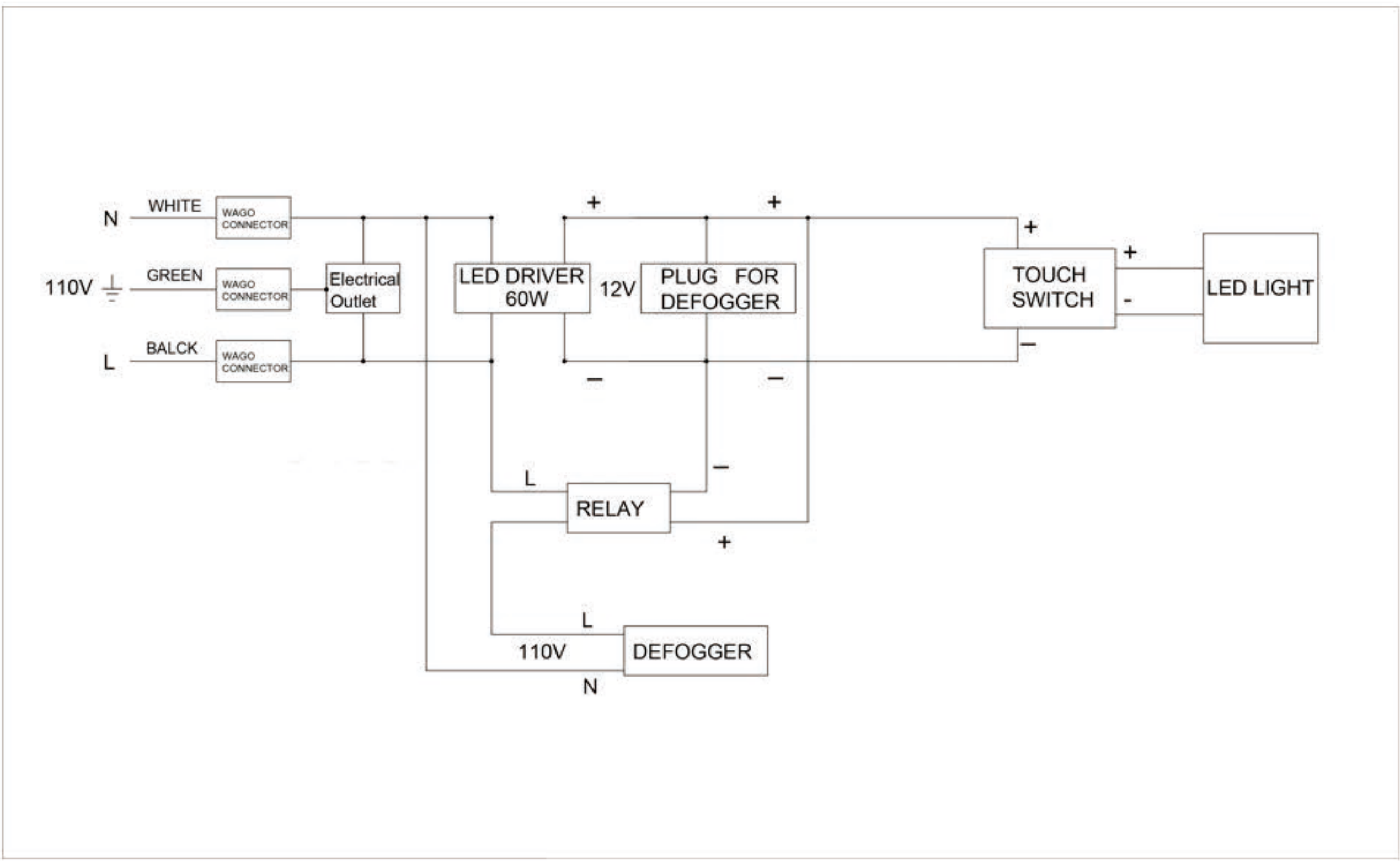
Circuit Diagram
