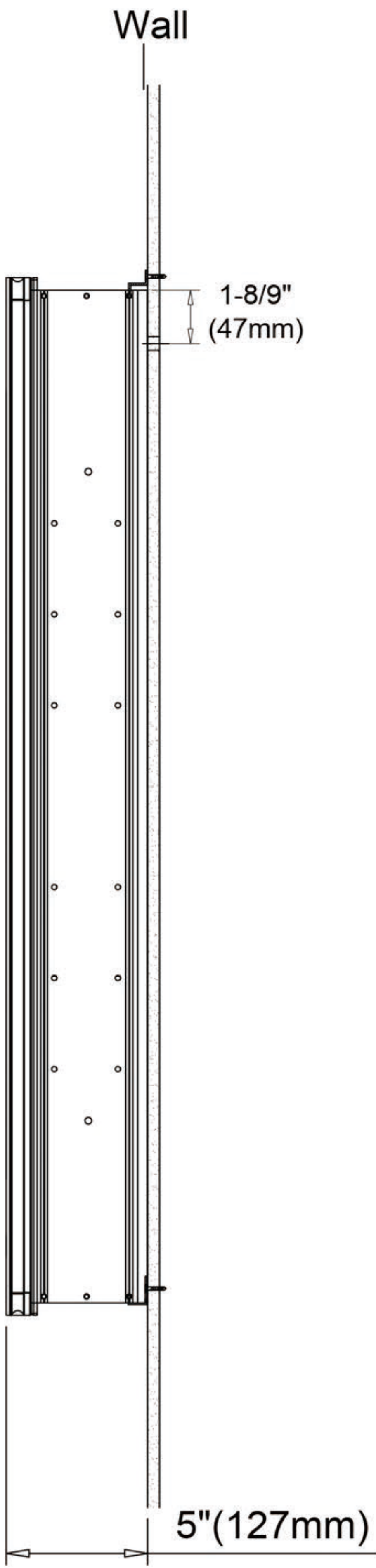
Surface Mount
