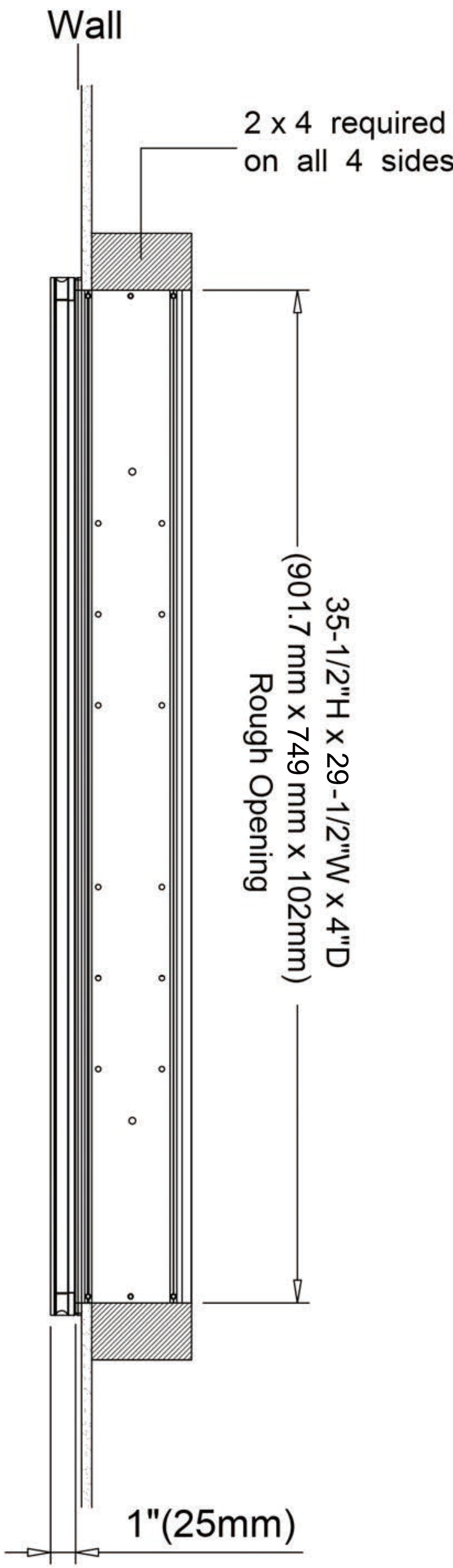
Recessed Mount
