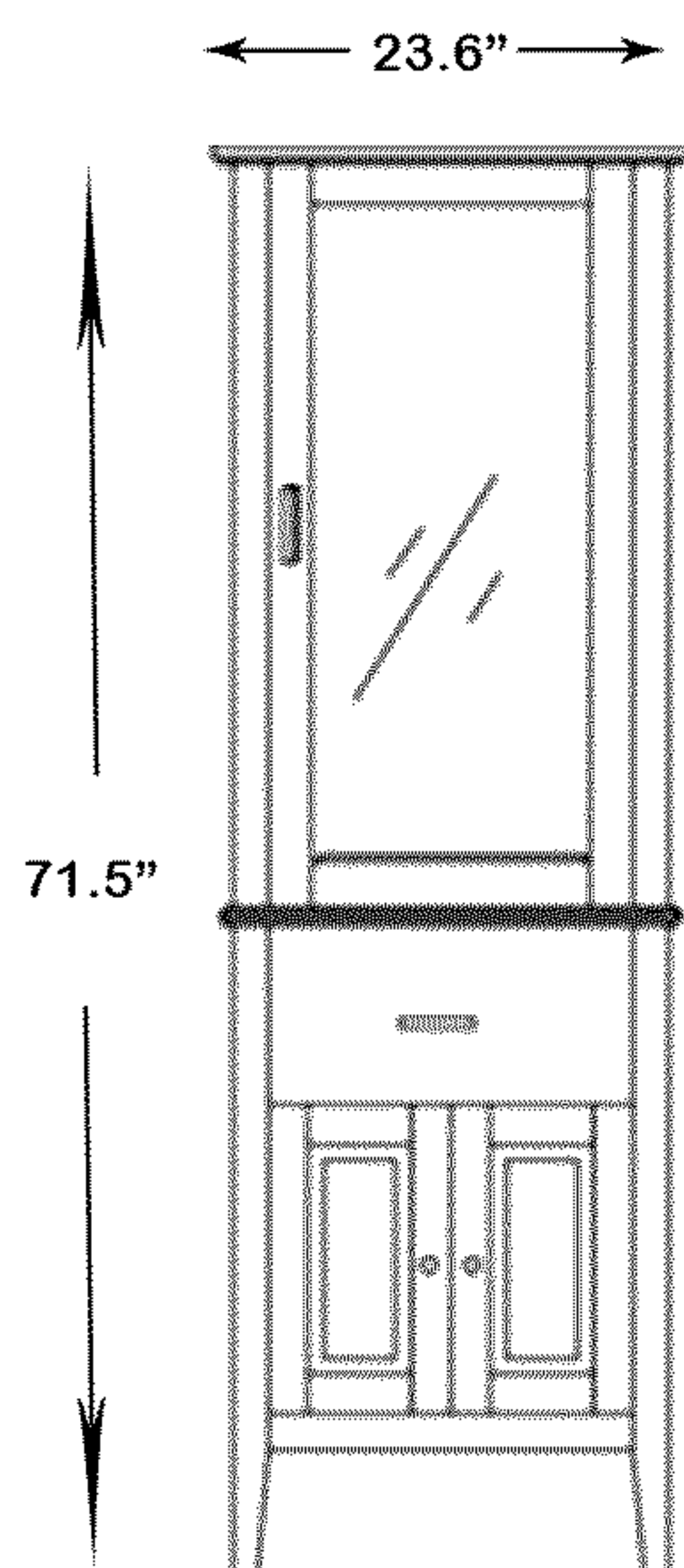
Cabinet Front
