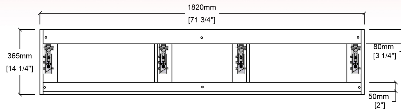
BACK VIEW
