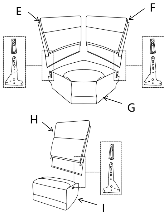
STEP 1: Assembly Backrest
