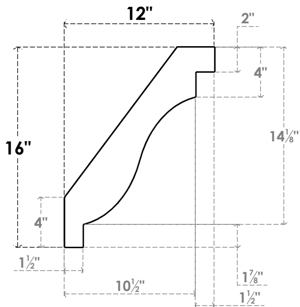
SIDE PROFILE
