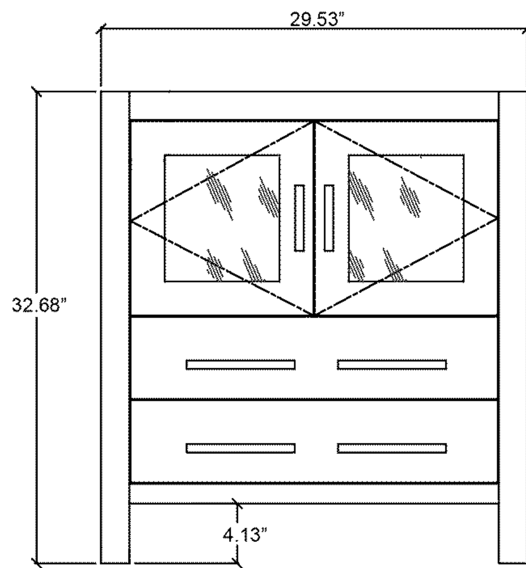
Front View
