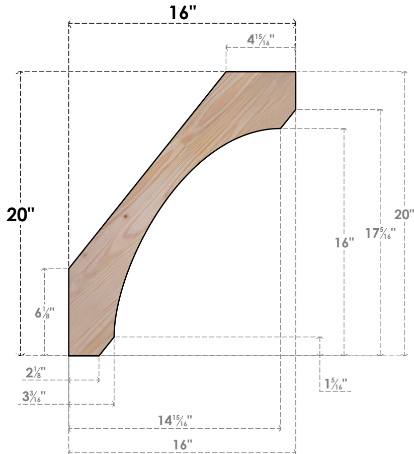
SIDE
