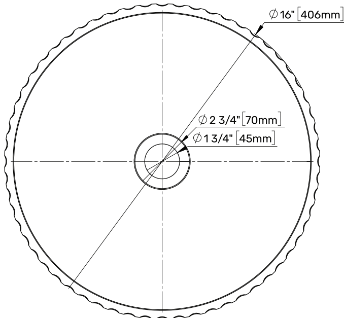
FRONT VIEW / VISTA FRONTAL / VUE DE FACE
