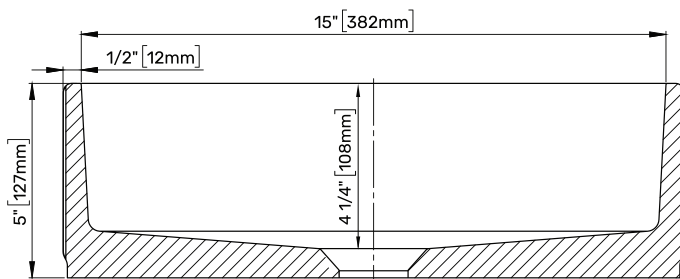
FRONT VIEW / VISTA FRONTAL / VUE DE FACE
