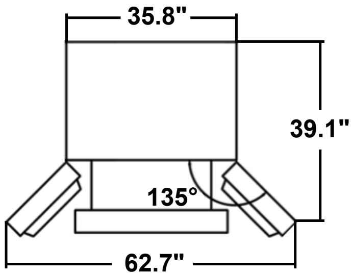
TOP VIEW, OPEN
