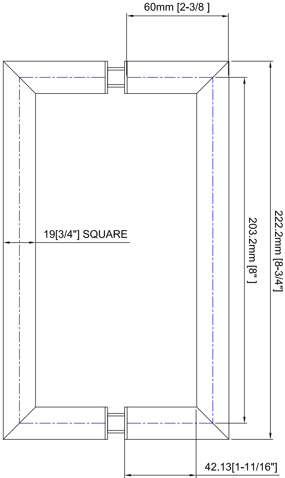
ROCKWELL CONTEMPORARY 8" BACK TO BACK HANDLE GLASS MOUNT FITS 1/4" TO 1/2" THICK GLASS DOORS
