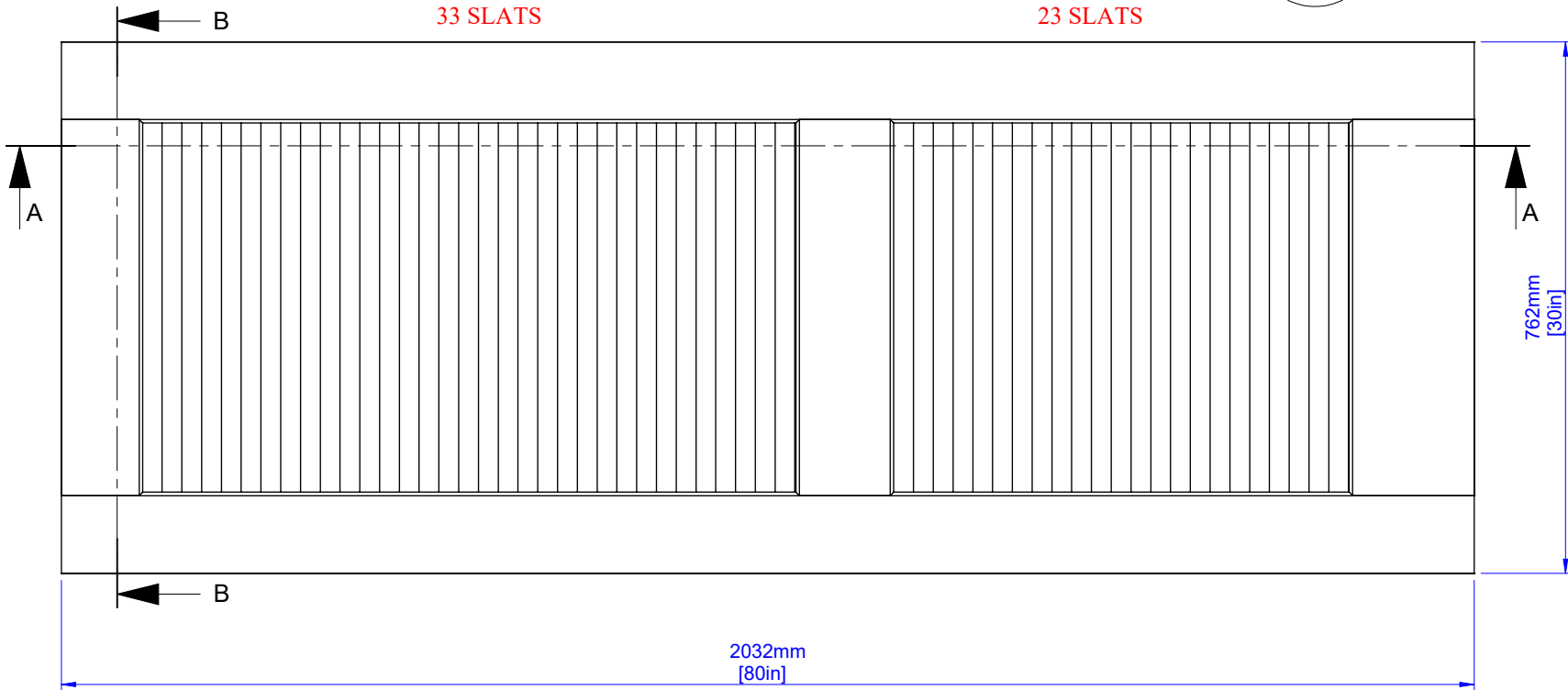
CLASSIC LOUVER 35mm (1 3/8") Louver/Louver Standard Ovolo Sticking 5mm Slats (28,5mm Pitch) Open
