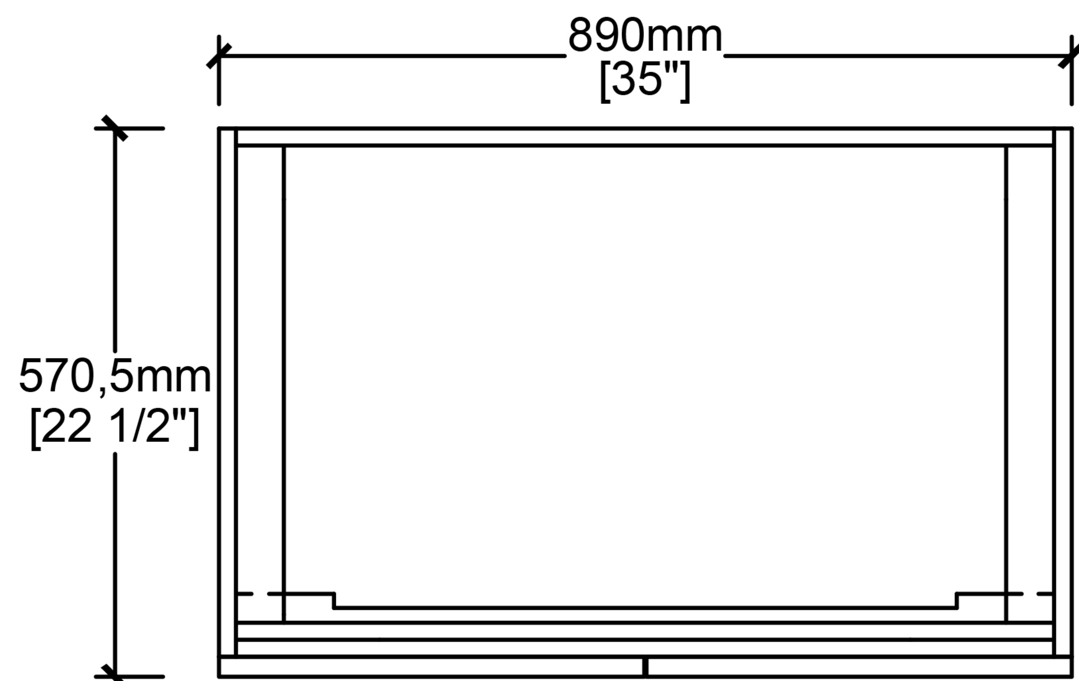
Top View
