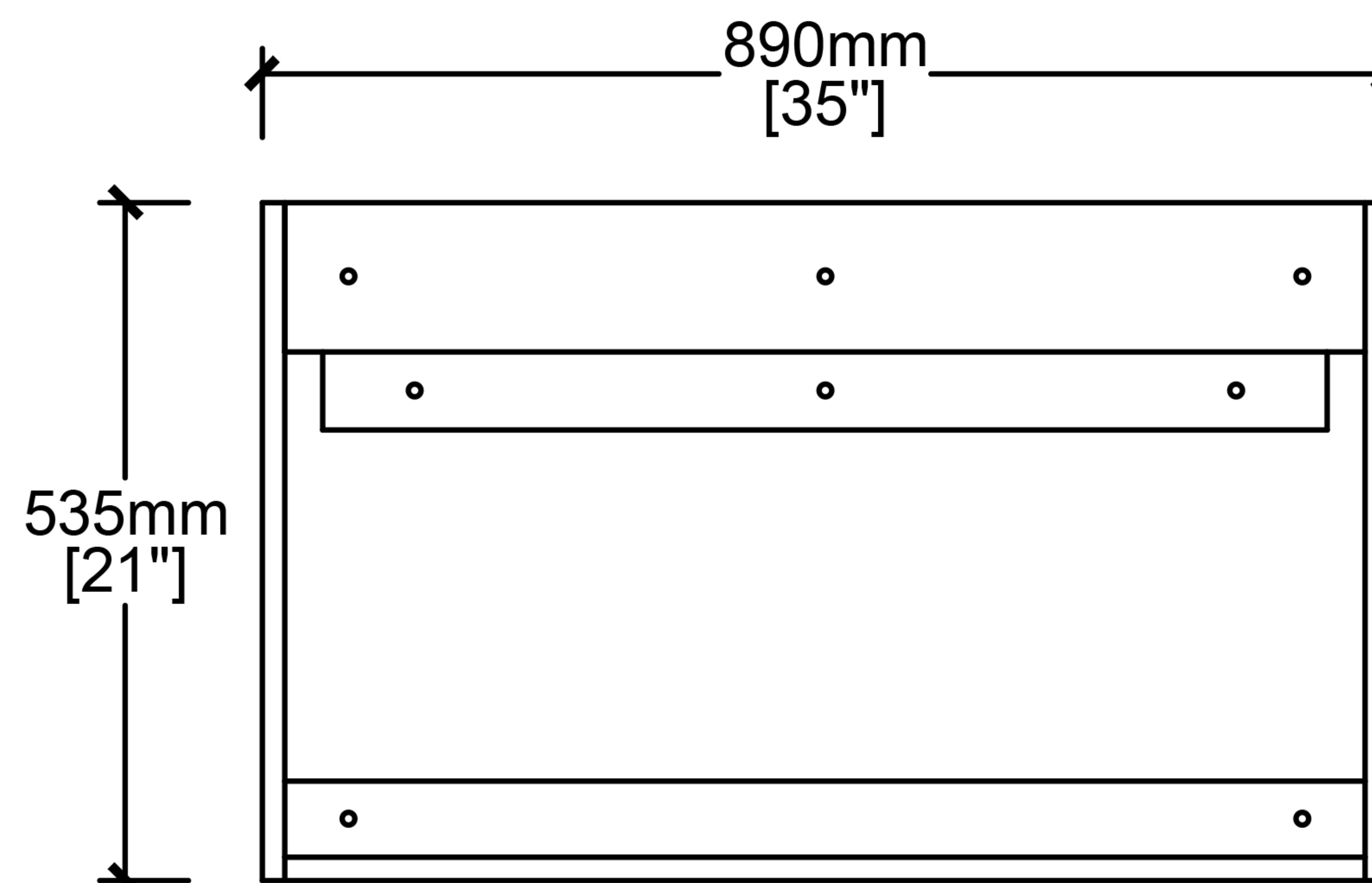
Top View
