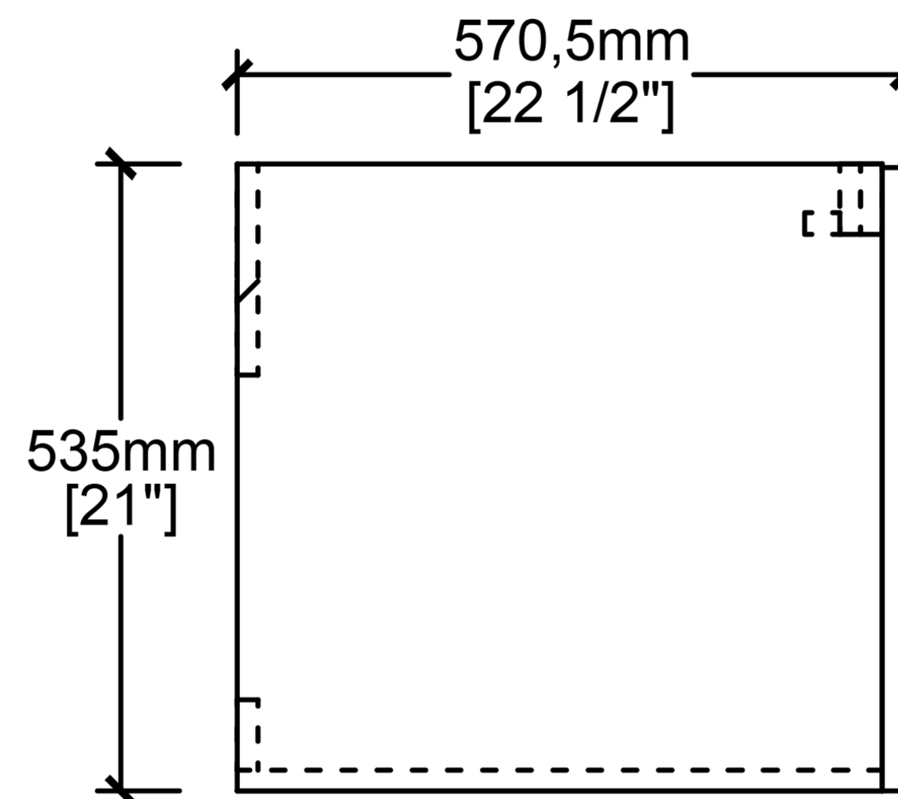
Side View
