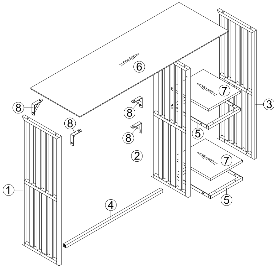
Exploded View
