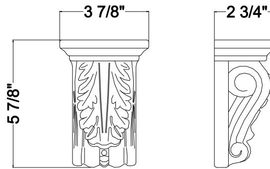
ITEM NUMBER:COR03X02X05LE 3 7/8"W x 2 3/4"D x 5 7/8"H Legacy Acanthus Corbel
