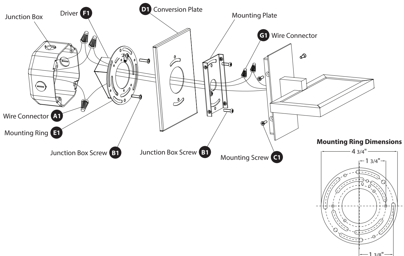
FIG. 2 MOUNT ON JUNCTION BOX
