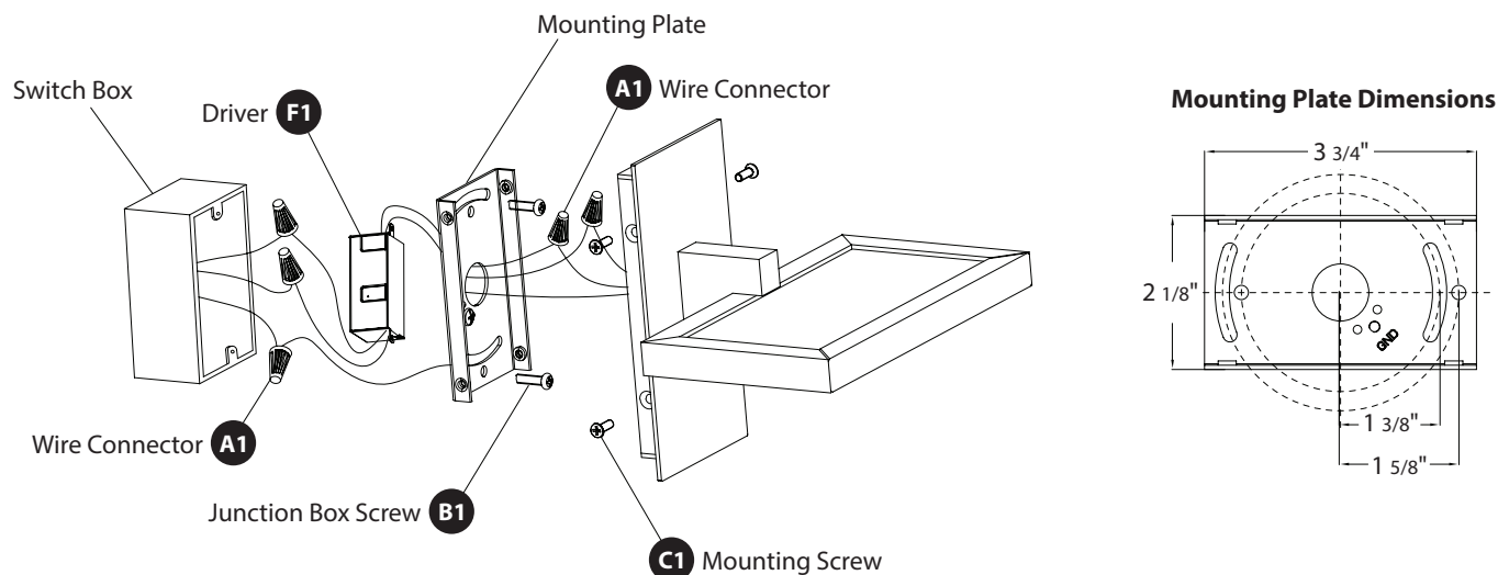
FIG. 1 MOUNT ON SWITCH BOX
