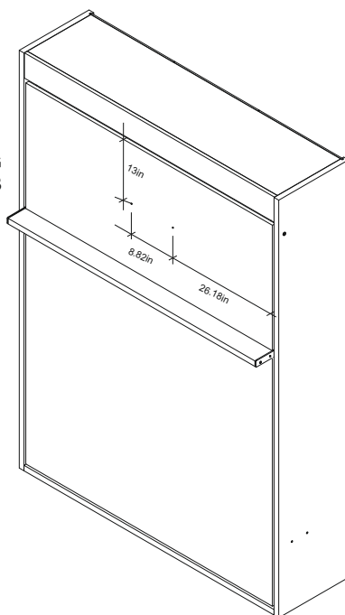
HANDLE MOUNTING OPTION B
