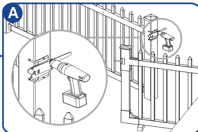
A - Align and fasten the gate latch catch to fit and function with the gate finger.
