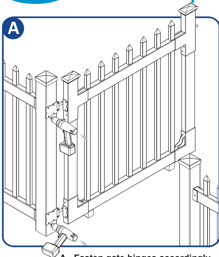
A - Fasten gate hinges accordingly
