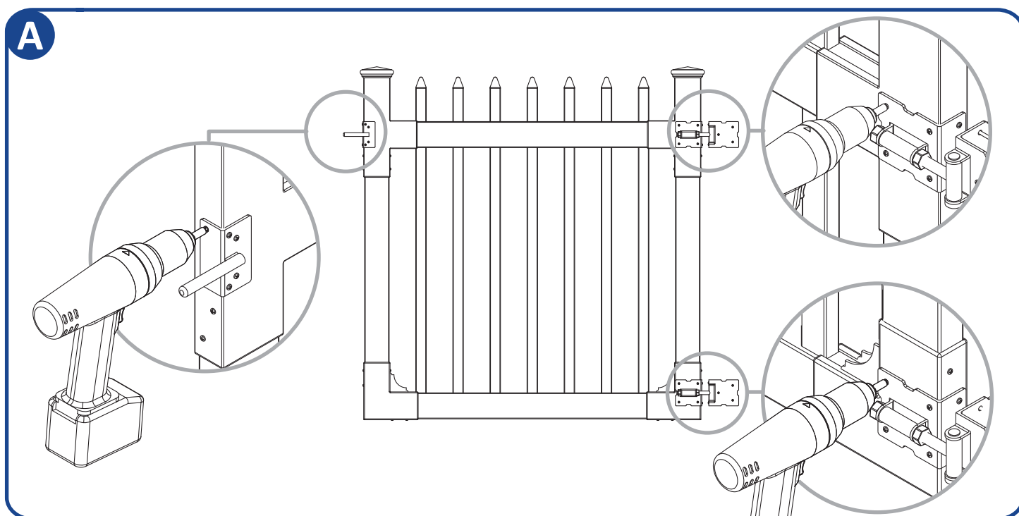
A - Fasten gate hinges and gate latch onto the gate brackets with screws.
