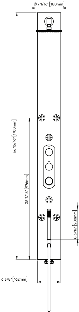
FRONT VIEW / VISTA FRONTAL / VUE DE FACE
