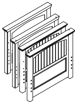
Wood Hole cover (4 PCS) BED ENDS (4 PCS)
