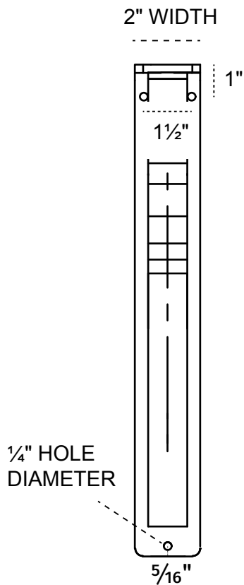
FRONT PROFILE
