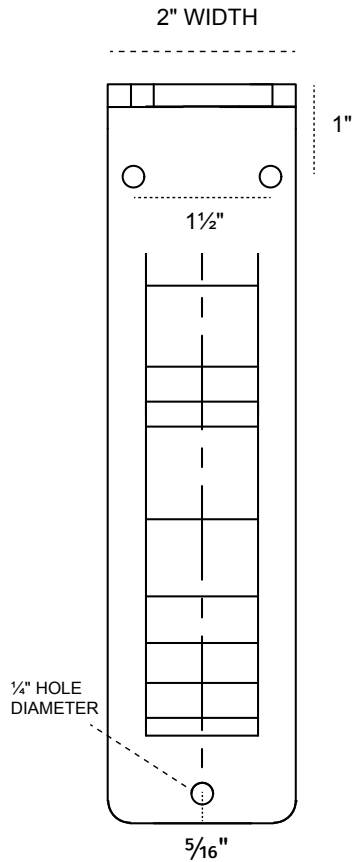
FRONT PROFILE
