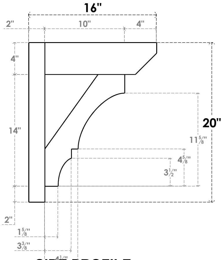
SIDE PROFILE
