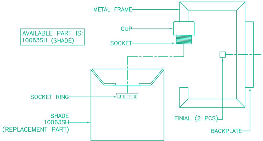
SIDE VIEW
