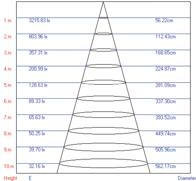
Lux-Distance Curve
